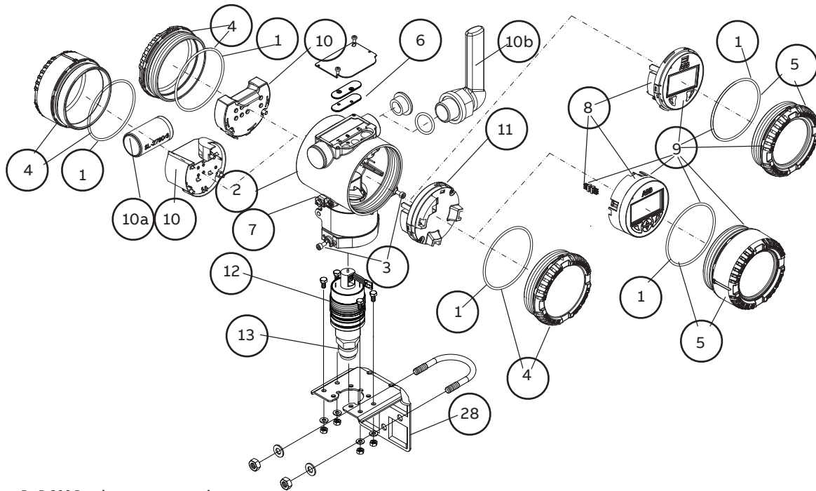
Figure 5 P-300 P style pressure transmitter
