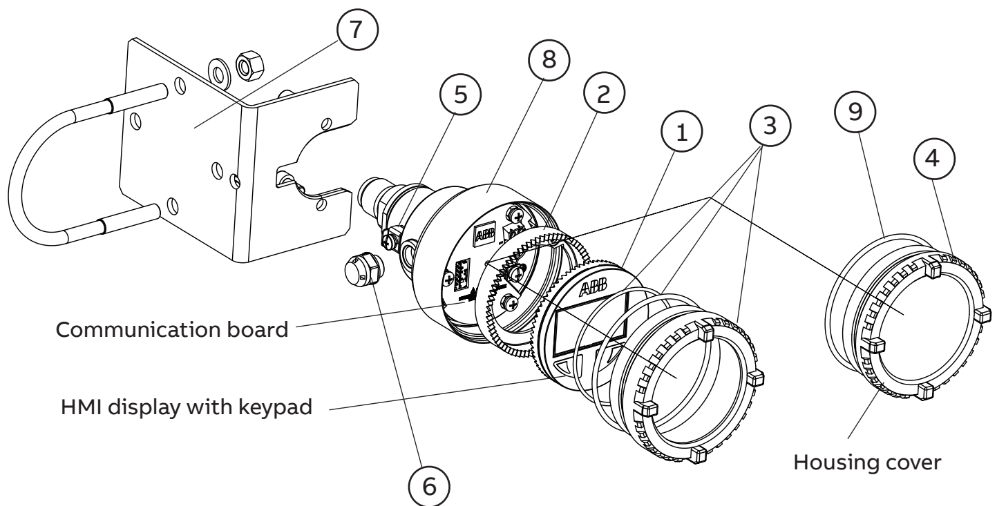
Figure 2 P-100 pressure transmitter
