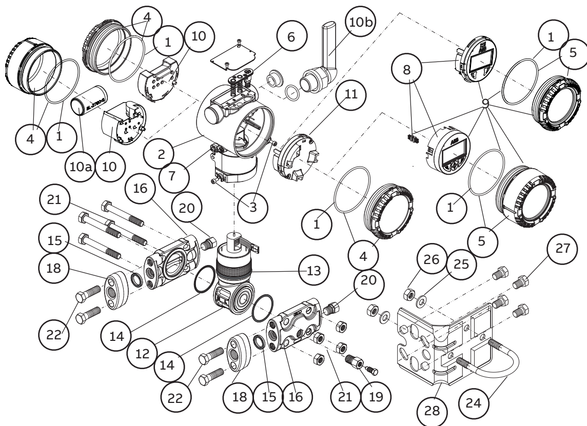
Figure 4 P-300 DP style pressure transmitter
