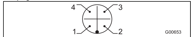
Fig. 44: Assignment for connection using optional M12 plug-in connector
