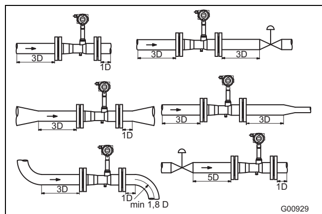
Fig. 9: Recommended inflow and outflow sections
