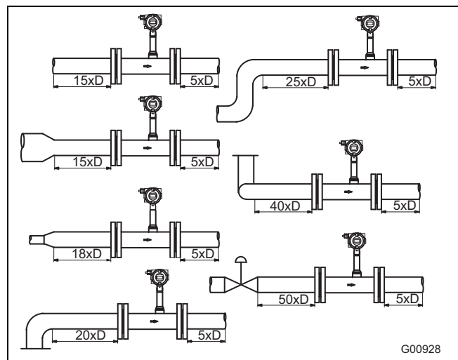
Fig. 8: Recommended inflow and outflow sections
