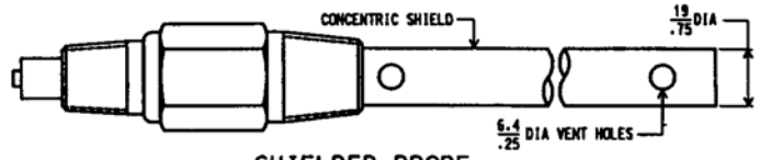
SHIELDED PROBE
