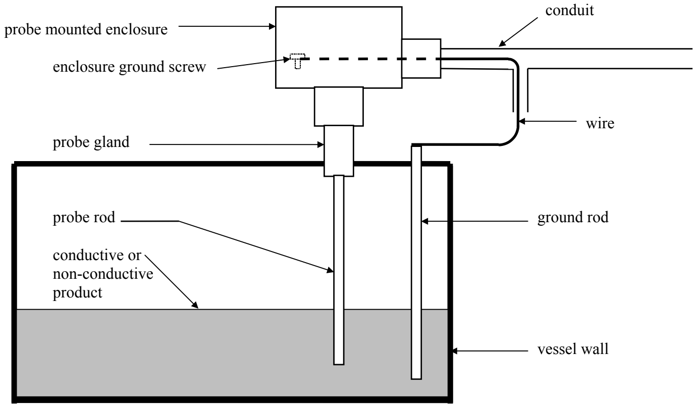
CUSTOMER INSTALLED GROUND ROD EMPLOYED
