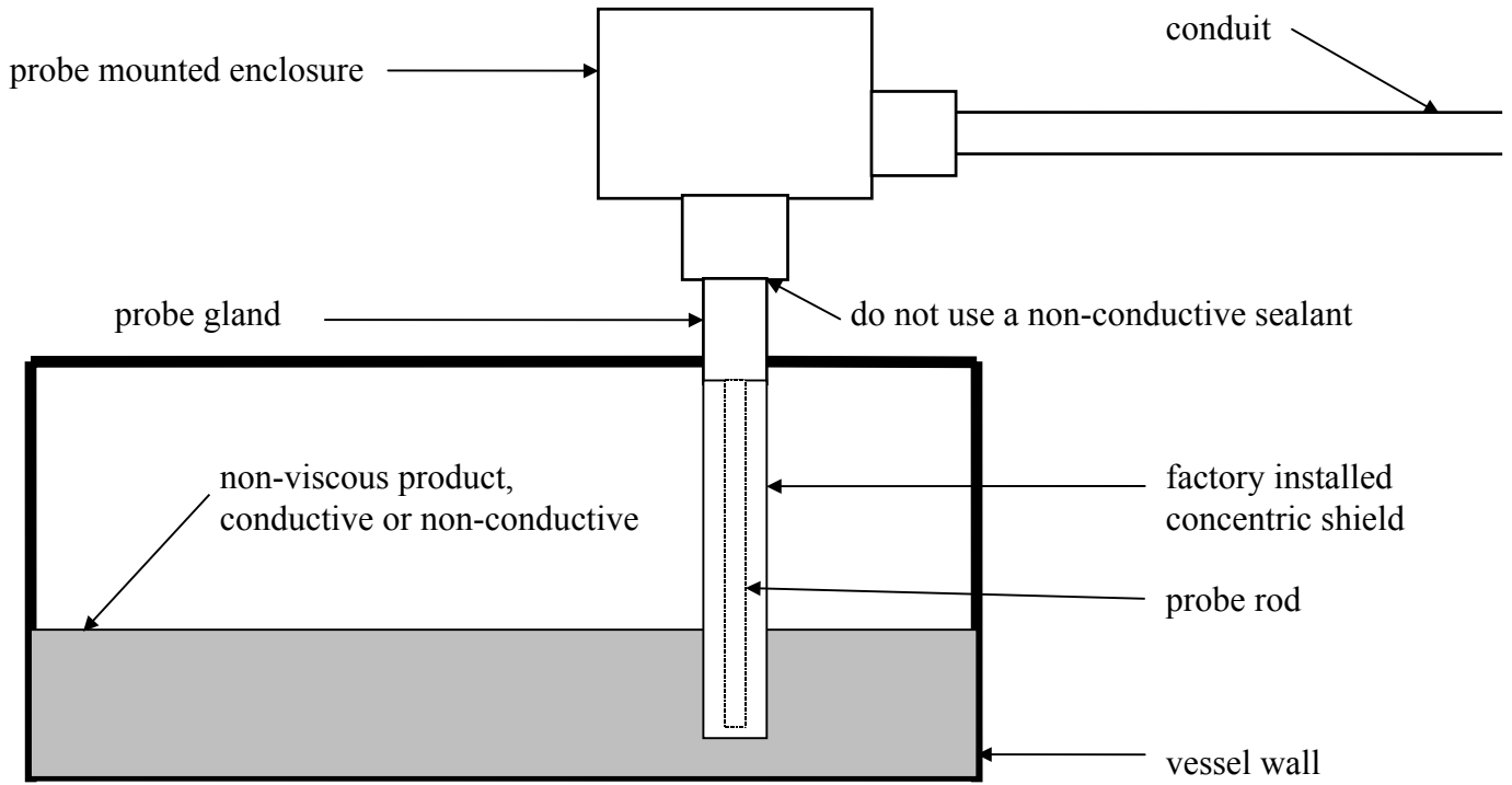
PROBE WITH CONCENTRIC SHIELD GROUNDING
