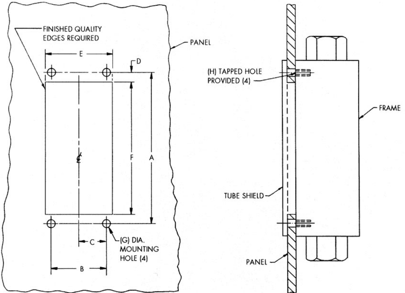
PANEL MOUNTING CUTOUT
